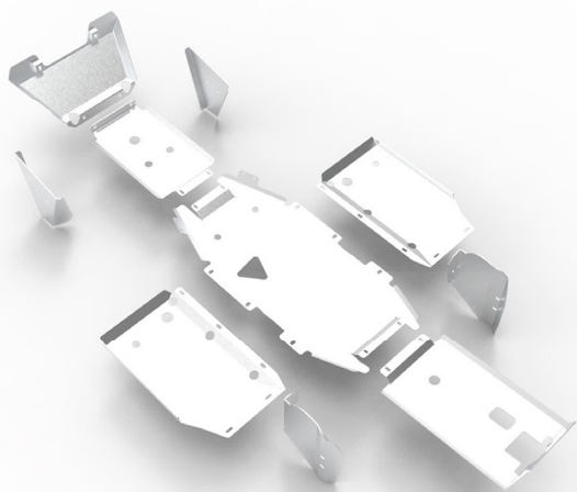
SET PLAQUE DE PROTECTION ALUMINIUM SKID PLATE FULL SET ALUMINIUM UCL-C625-07
