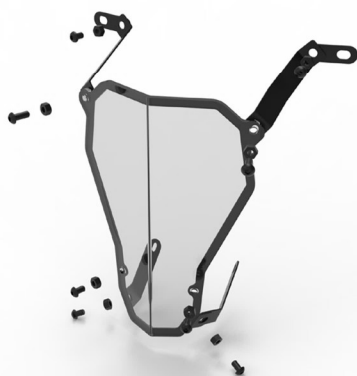
PROTECTION PHARE EN PLEXIGLASS PLEXI HEADLIGHT PROTECTION UCL-NK250-RK-09
